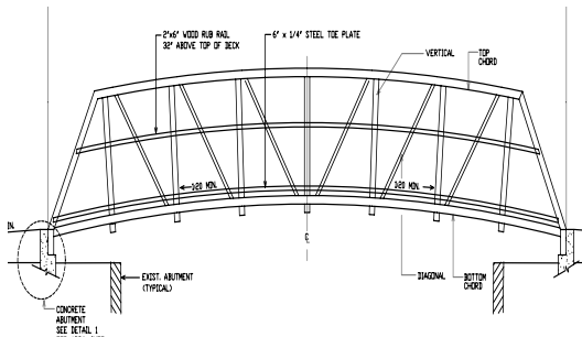
A drawing showing what the completed pedestrian bridge is going to look like.
